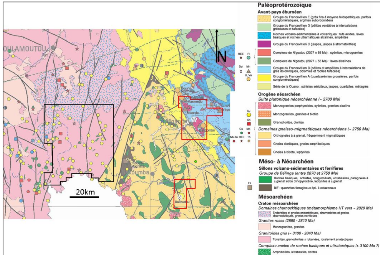
Figure 2 : Extract of a geological map of Gabon at a scale of 1:1,000,000 from SYSMIN 2009
